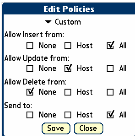
Figure 6 Privacy policy specification: Definition
